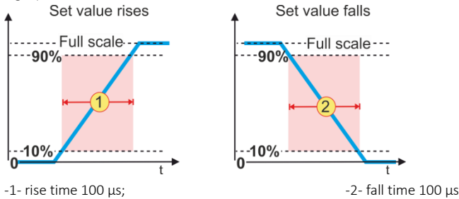
Fig. 4) Slew rate at a resistive load
