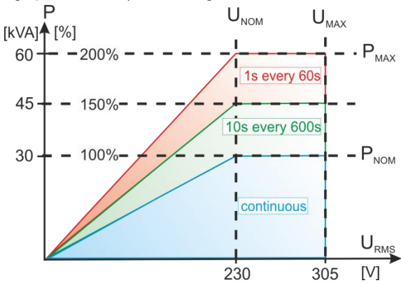
Fig. 3) Overloadability versus voltage
