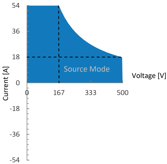
Figure 1: G5.SRC.9.500.54, voltage/current operating area.
