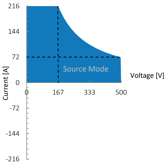
Figure 1: G5.SRC.36.500.216, voltage/current operating area.
