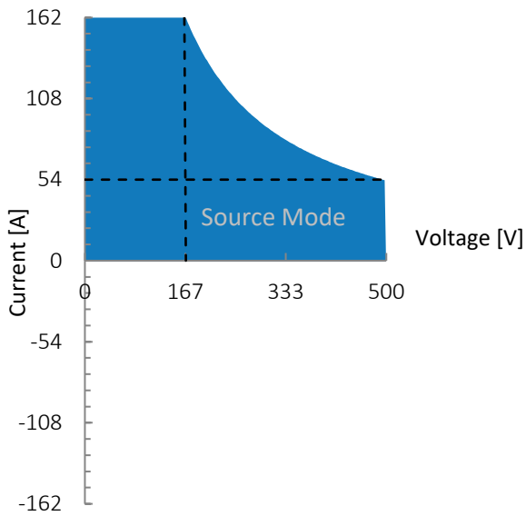
Figure 1: G5.SRC.27.500.162, voltage/current operating area.
