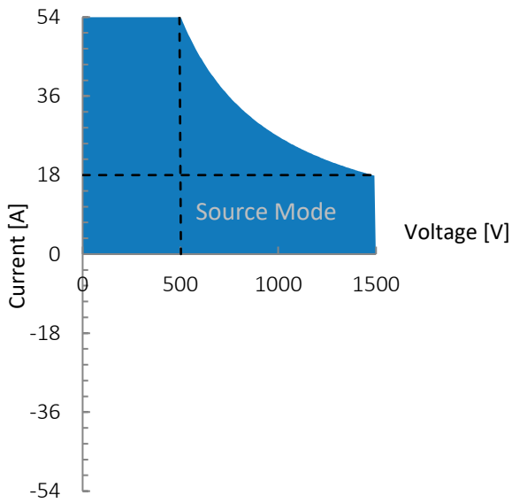
Figure 1: G5.SRC.27.1500.54, voltage/current operating area.
