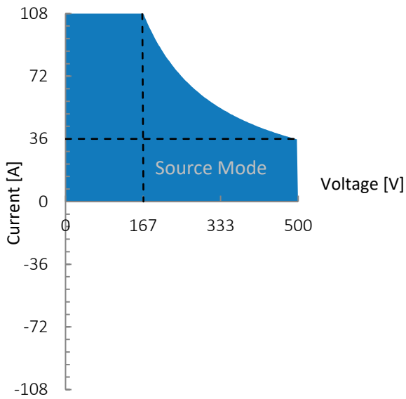
Figure 1: G5.SRC.18.500.108, voltage/current operating area.
