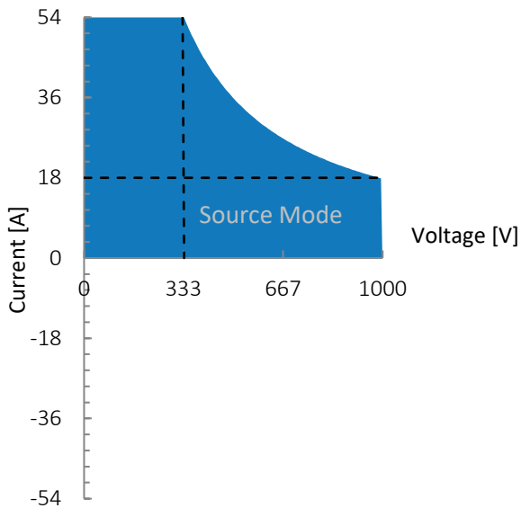
Figure 1: G5.SRC.18.1000.54, voltage/current operating area.
